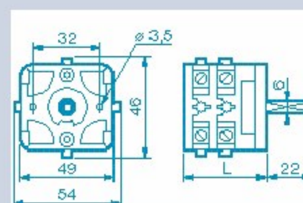
Mounting at back of box
