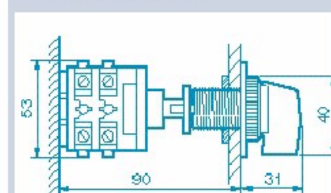
Mounting at back of box
