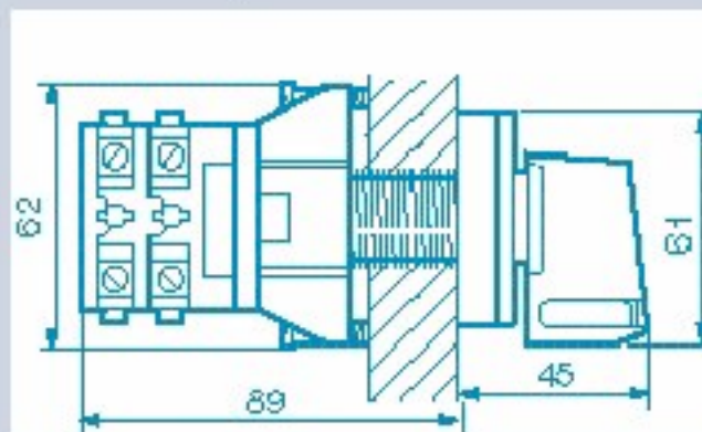
Mounting on the cover
